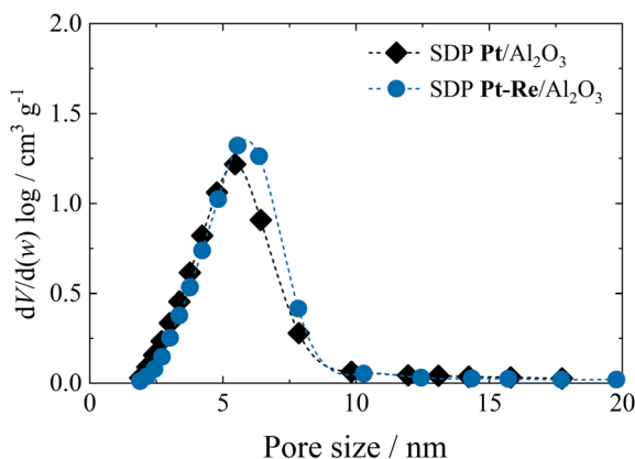
Fig. 5 Pore volume ( V_{\text{BHJ}} ) and pore size distribution (PSD) obtained for Pt/ \text{Al}_2\text{O}_3 (0.3 wt% Pt) and Pt-Re/ \text{Al}_2\text{O}_3 (0.3 wt% Pt, 0.27 wt% Re, Re/Pt = 0.88) via \text{N}_2 physisorption obtained using the adsorption branch.
