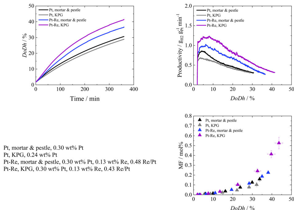
Fig. 13 Degree of dehydrogenation, \text{H}_2 productivity and methylfluorene (MF) formation during dehydrogenation of perhydro benzyltoluene (H12-BT) with solvent deficient precipitation (SDP) Pt/ \text{Al}_2\text{O}_3 and Pt-Re/ \text{Al}_2\text{O}_3 catalysts synthesised either with a mortar & pestle or with a core drawn precision glassware (KPG) mixer. Experimental conditions: T = 250^\circ\text{C} , p = 1 bara, n_{\text{LOHC}} = 0.1 mol, w_{\text{Pt}} = 0.3 wt%, n_{\text{Pt}}/n_{\text{LOHC}} = 0.0001 , t_{\text{R}} = 360 min, \dot{V}_{\text{Ar}} = 300 mL \text{min}^{-1} . DoDh and productivity data was obtained from TCD measurements, whereas product composition data was determined via GC method.
