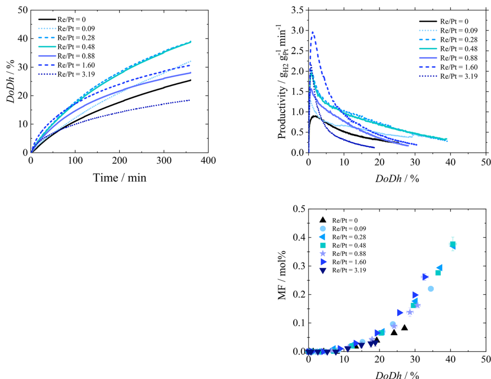
Fig. 10 Degree of dehydrogenation, \text{H}_2 productivity and methylfluorene (MF) formation during semi-batch dehydrogenation of perhydro benzyltoluene (H12-BT) with solvent deficient precipitation (SDP) Pt-Re/ \text{Al}_2\text{O}_3 catalysts with different Re/Pt molar ratios. Experimental conditions: T = 250^\circ\text{C} , p = 1 bara, n_{\text{LOHC}} = 0.1 mol, w_{\text{Pt}} = 0.3 wt%, n_{\text{Pt}}/n_{\text{LOHC}} = 0.0001 , t_{\text{R}} = 360 min, \dot{V}_{\text{Ar}} = 300 \text{ mL}_{\text{N}} \text{ min}^{-1} . DoDh and productivity data was obtained from TCD measurements, whereas product composition data were determined via the GC method. Average values and standard deviation are shown.
