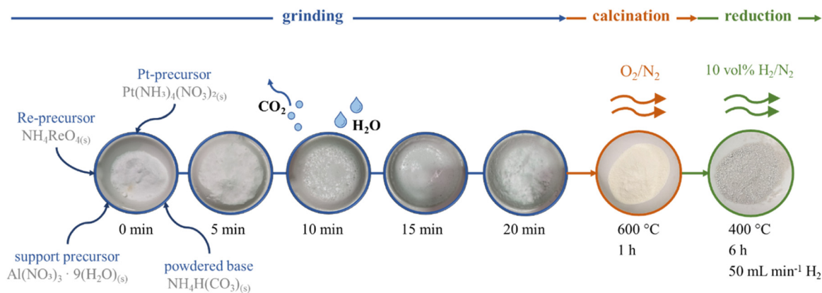
Fig. 1 Summary of synthesis of a Pt-Re/Al 2 O 3 via the solvent deficient precipitation (SDP) method, showing the grinding, calcination and reduction steps.
